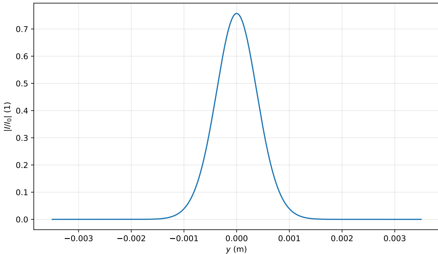
Intensity profile I(x=0, y, z=1.433)/I_0 , P_{in}=0.2P_{cr} , artificial time
